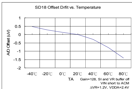
Figure 6.8-1l SD18 Offset Temperature drift
